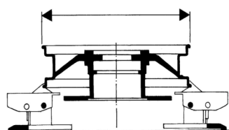
Ruote moto con freno disco e trasmissione a cinghia Motorcycle wheels with brake disk and belt drive
